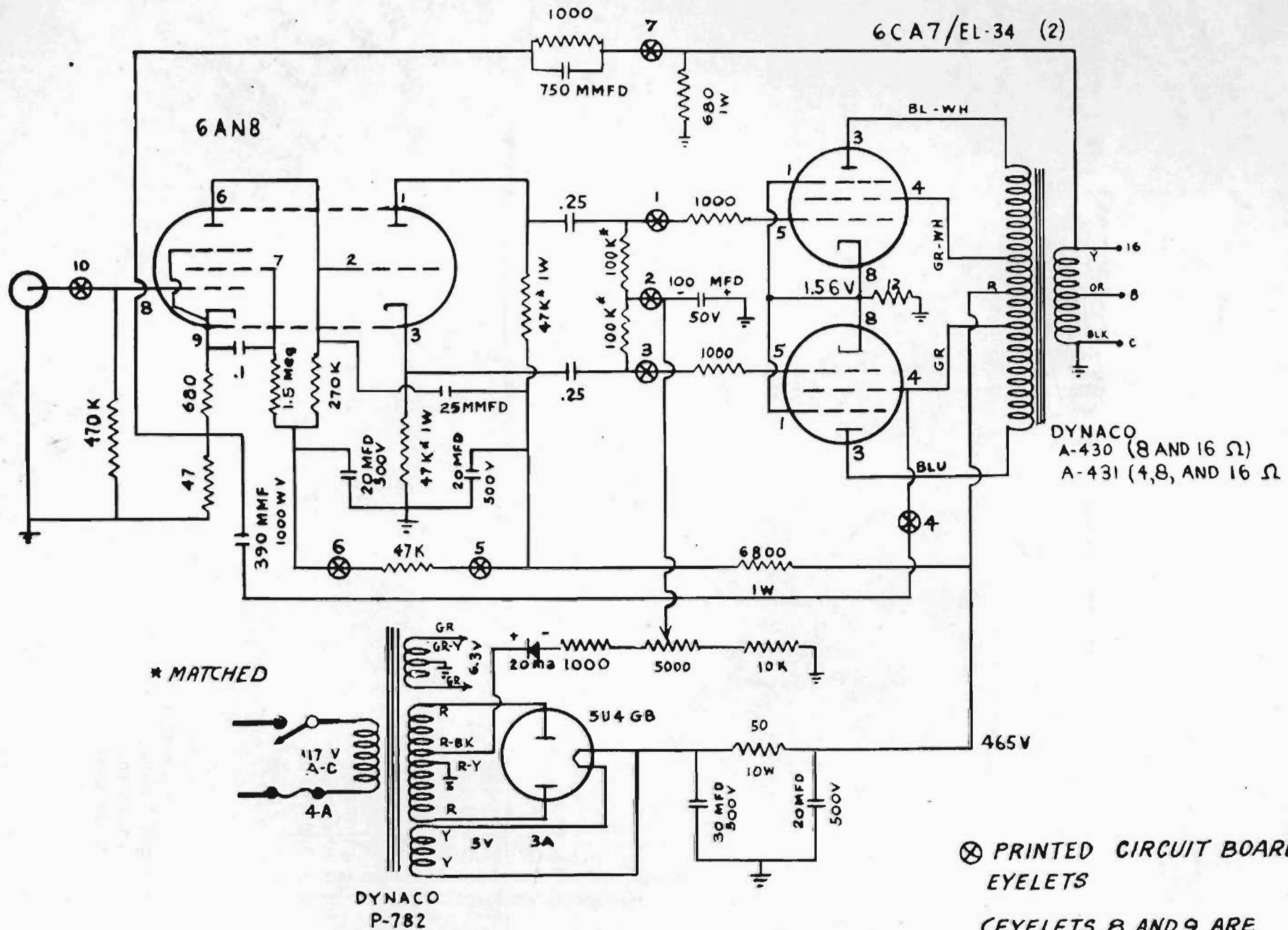
DYNACO CIRCUIT AS USED IN THE DYNAKIT
