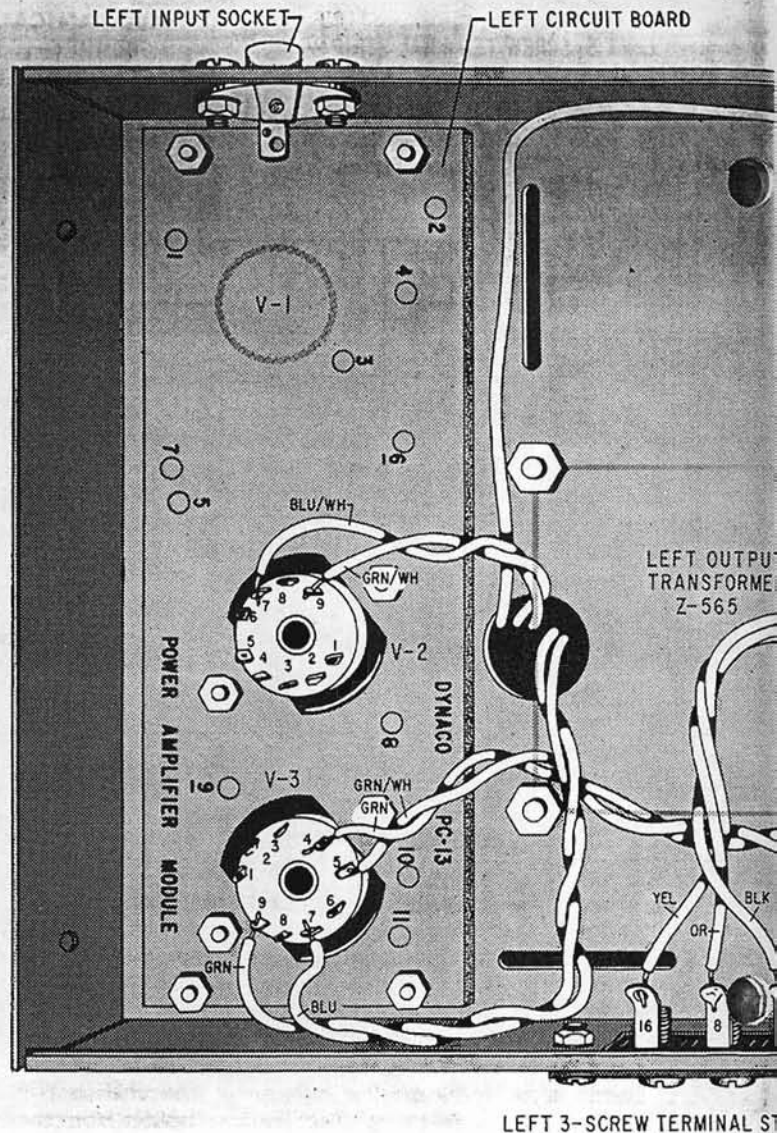
LEFT 3-SCREW TERMINAL STRIP
